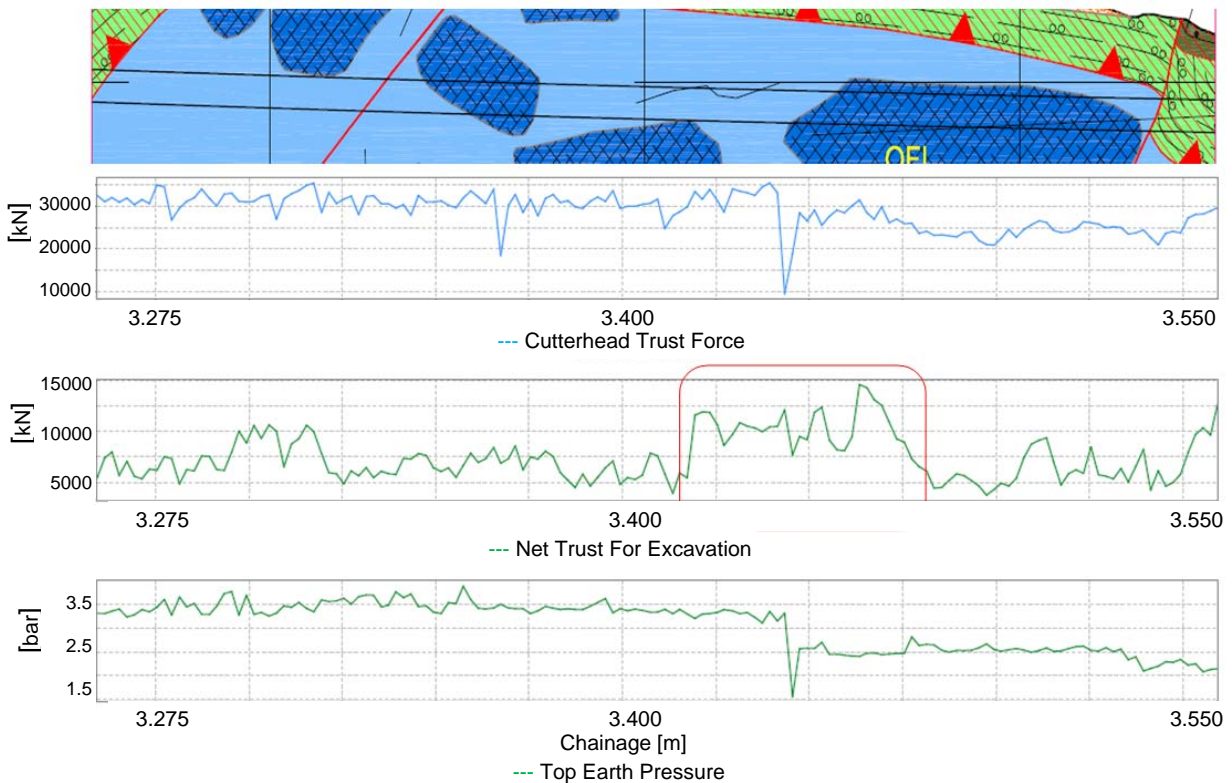
Figure 5. Variability of the “Net Thrust for Excavation”.
