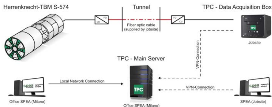
Figure 2. Network Setup
