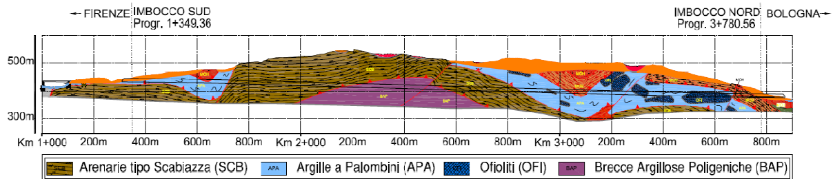
Figure 1. Geological section of the Sparvo tunnel
